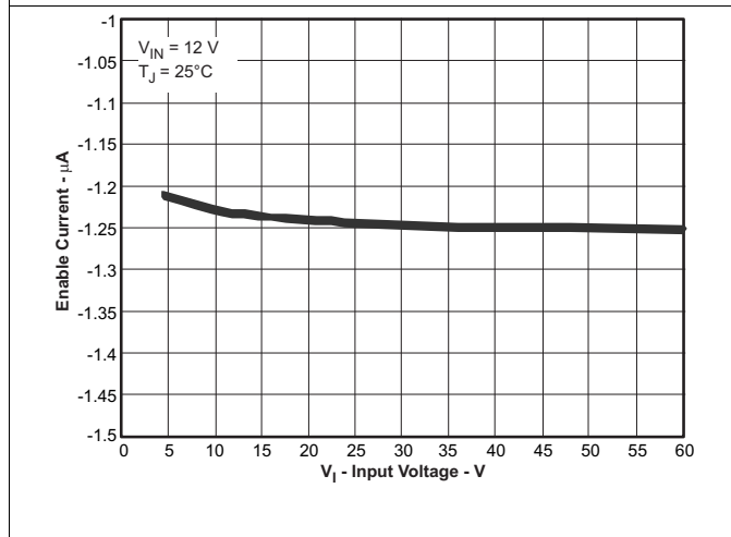
Figure 11. Enable Pin Pullup Current vs Input Voltage
