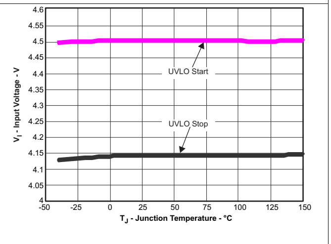
Figure 10. Input Voltage (UVLO) vs Temperature
