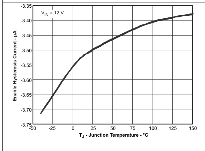
Figure 9. Enable Pin Hysteresis Current vs Temperature
