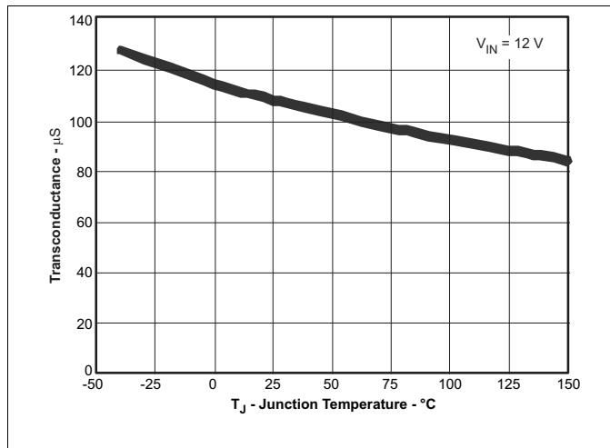
Figure 7. Error Amp Transconductance vs Temperature
