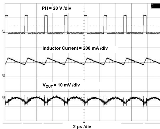
Figure 36. Output Ripple in CCM
