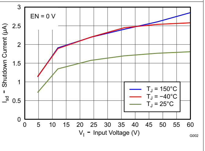
Figure 12. Shutdown Supply Current (VIN) vs Input Voltage
