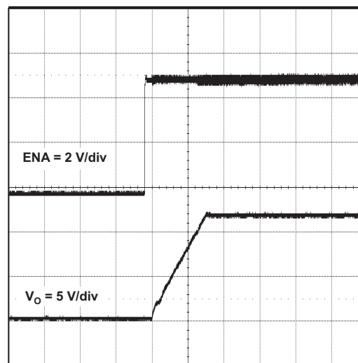
Figure 20. Startup Waveform, ENA and V_O
