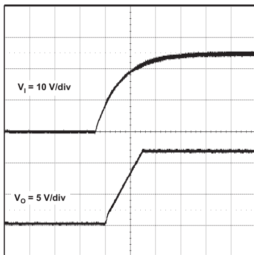
Figure 19. Startup Waveform, V_I and V_O
