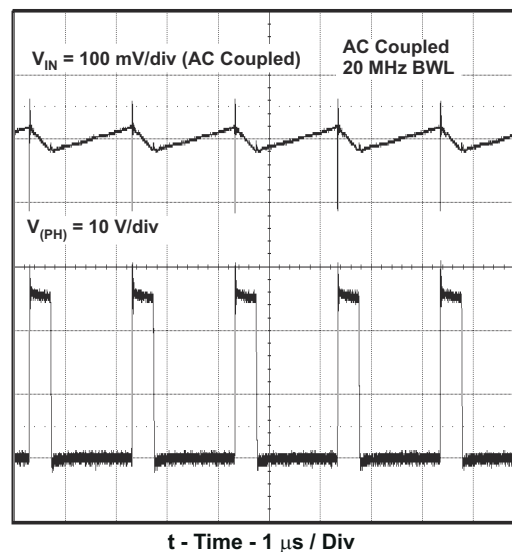
Figure 8-16. Input Voltage Ripple and PH Node, I_O = 1 A
