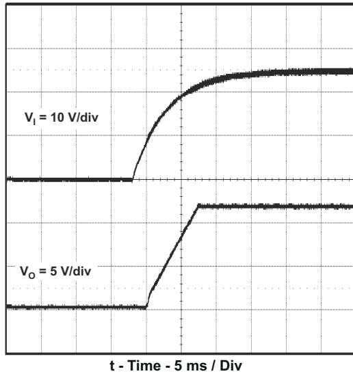
Figure 8-11. Startup Waveform, V_I and V_O
