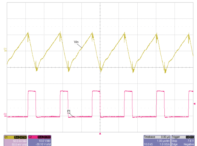
Figure 18. Input Ripple
