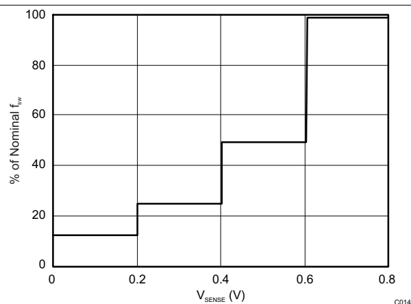
Figure 11. Switching Frequency vs V_{\text{SENSE}}
