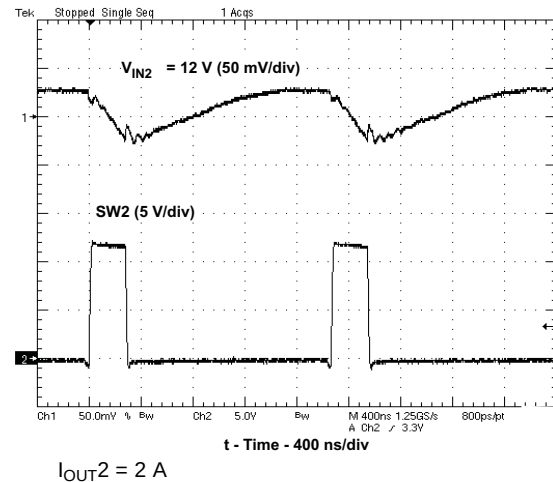
Figure 24. V_{IN2} Input Voltage Ripple
