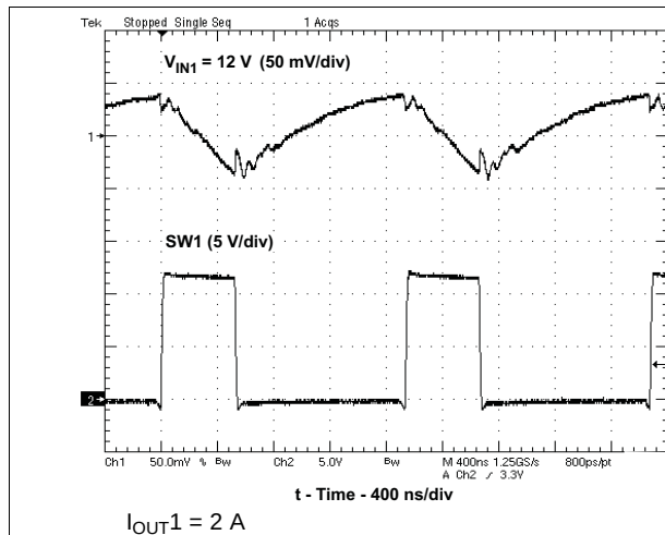
Figure 23. V_{IN1} Input Voltage Ripple
