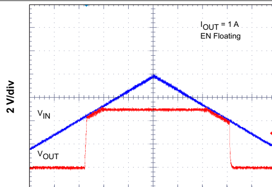
Time = 40 \mu s/div Figure 60. Low Dropout Operation
