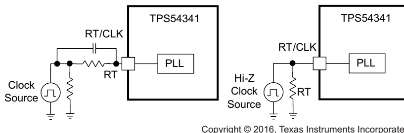
Figure 38. Synchronizing to a System Clock
