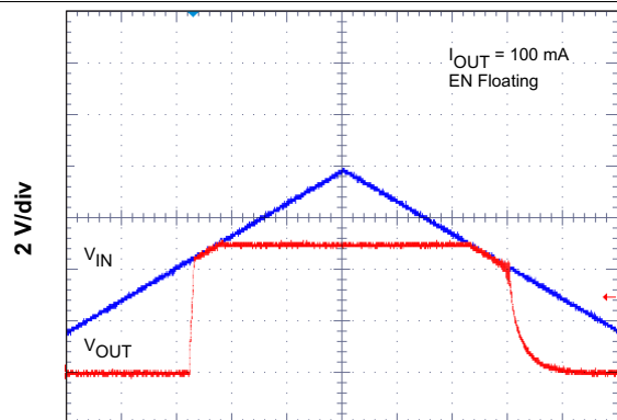
Time = 40 \mu s/div Figure 59. Low Dropout Operation
