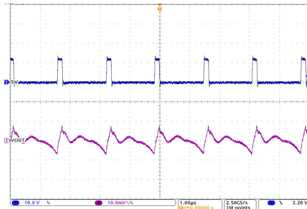
Figure 8-14. Output Voltage Ripple, 600 kHz FCCM, 35-A Load
