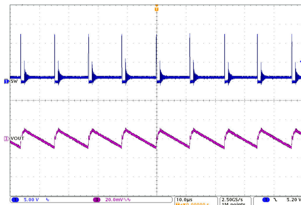
Figure 8-18. Output Voltage Ripple, DCM, 500-mA Load
