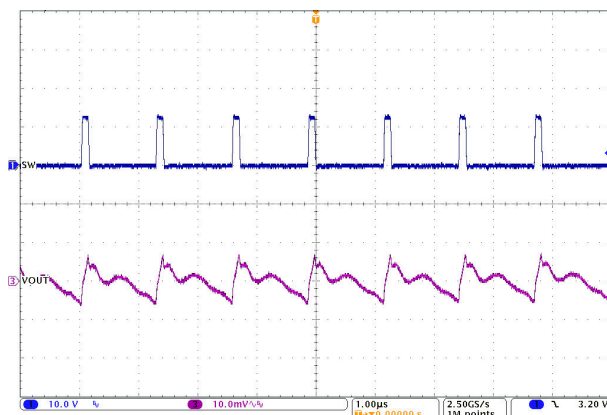
Figure 8-16. Output Voltage Ripple, FCCM, No load
