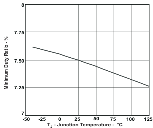
Figure 6-8. Minimum Controllable Duty Ratio vs Junction Temperature
