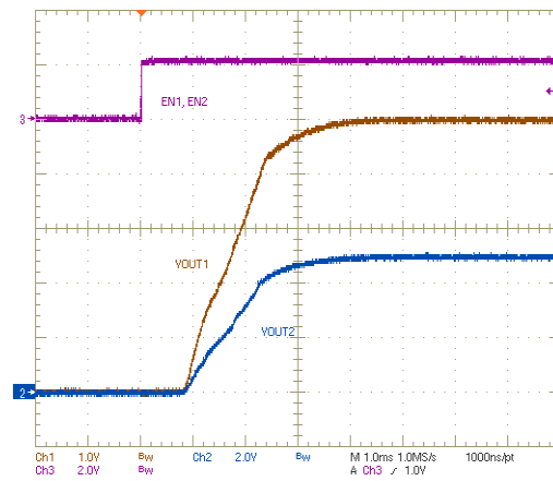
Figure 7-7. Ratio-Metric Startup using Coupled SS/TR pins
