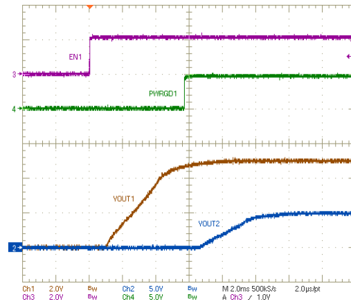
Figure 7-5. Sequential Startup using EN and PWRGD
