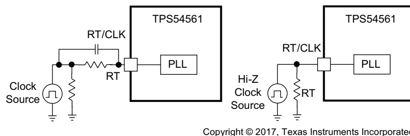
Figure 7-12. Synchronizing to a System Clock
