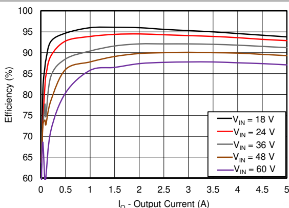
V_{OUT} = 12\text{ V} f_{SW} = 800\text{ kHz} Figure 8-22. Efficiency vs Output Current
