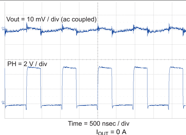
Figure 45. Output Ripple
