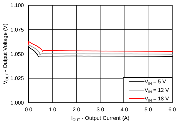
Figure 5. 1.05-V Output Voltage vs Output Current
