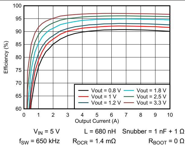
Figure 5-2. TPS546A24S Efficiency vs Output Current
