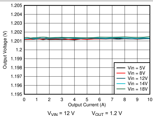
Figure 7-3. Load Regulation
