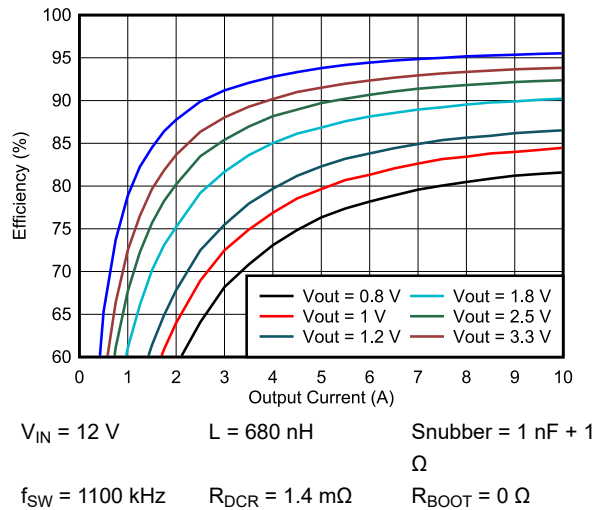
Figure 5-5. TPS546A24S Efficiency vs Output Current
