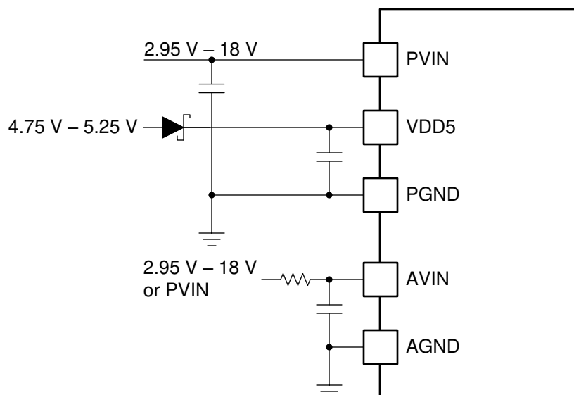
Figure 6-4. TPS546A24S Separate PVIN, AVIN, and VDD5 Connections
