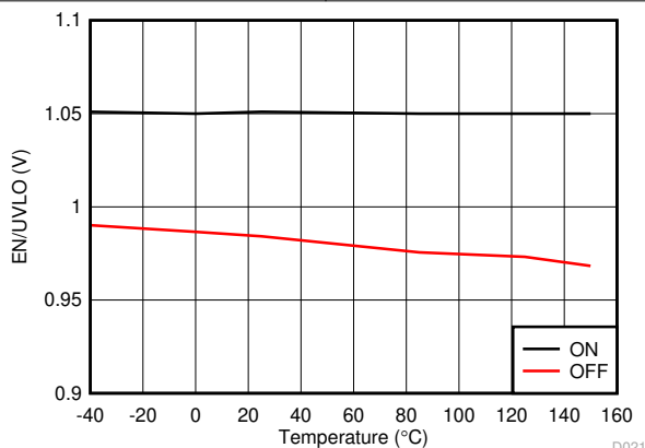
Figure 5-15. EN/UVLO Thresholds vs Junction Temperature
