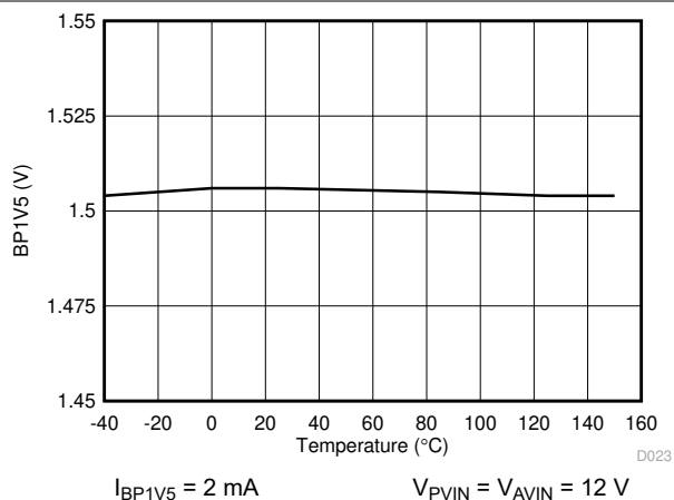
Figure 5-12. BP1V5 Voltage vs Junction Temperature
