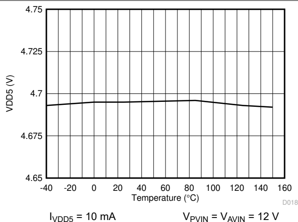
Figure 5-11. VDD5 Voltage vs Junction Temperature
