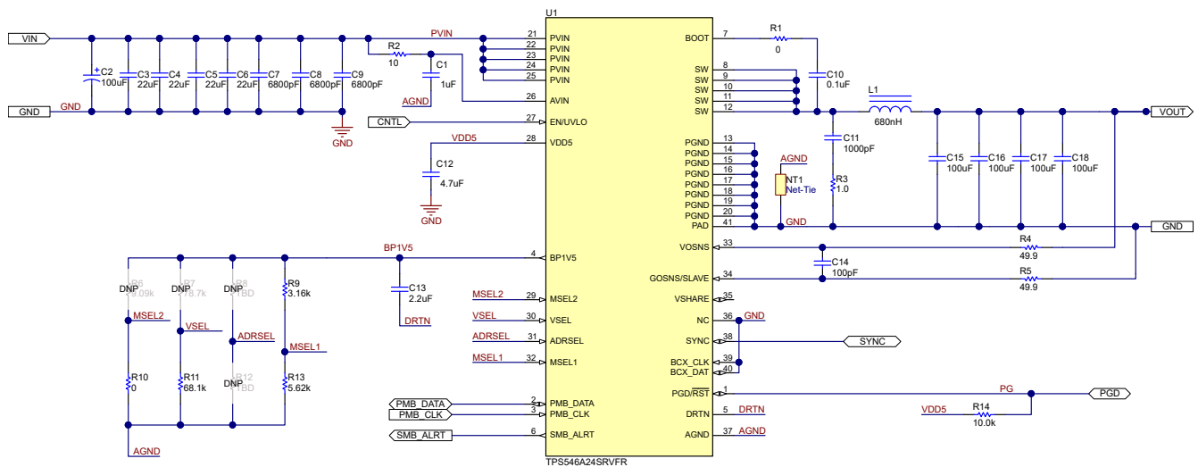
Figure 7-1. TPS546A24S Application
