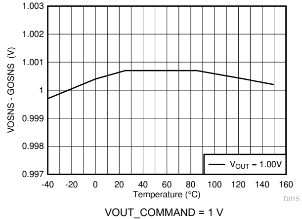
Figure 5-8. Output Voltage vs Junction Temperature
