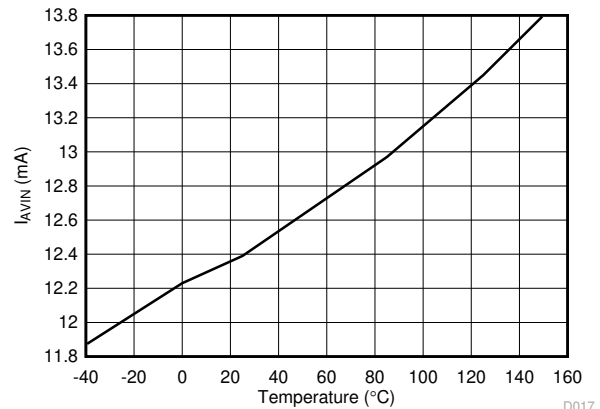
Figure 5-10. Non-Switching Input Current ( I_{AVIN} ) vs Junction Temperature
