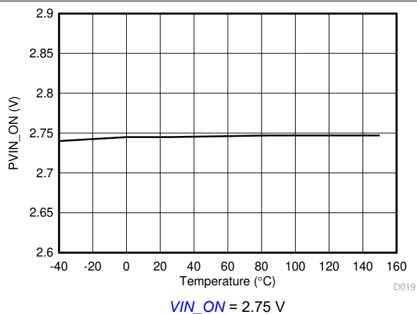
Figure 5-13. Turnon Voltage vs Junction Temperature
