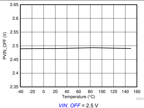
Figure 5-14. Turnoff Voltage vs Junction Temperature
