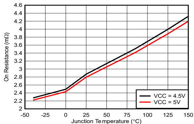
Figure 5-2. High-Side MOSFET On-Resistance ( R_{DS(on)} ) vs Junction Temperature
