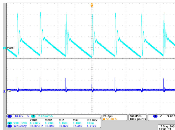
Figure 8-4. Output Voltage Ripple, 1.2V Vout, 800kHz DCM, No Load
