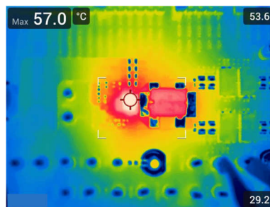
Figure 8-7. Thermal Characteristics, 800kHz FCCM, External 5V Bias, 25A Load
