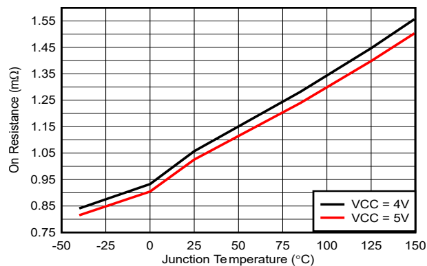
Figure 5-1. Low-Side MOSFET On-Resistance ( R_{DS(on)} ) vs Junction Temperature
