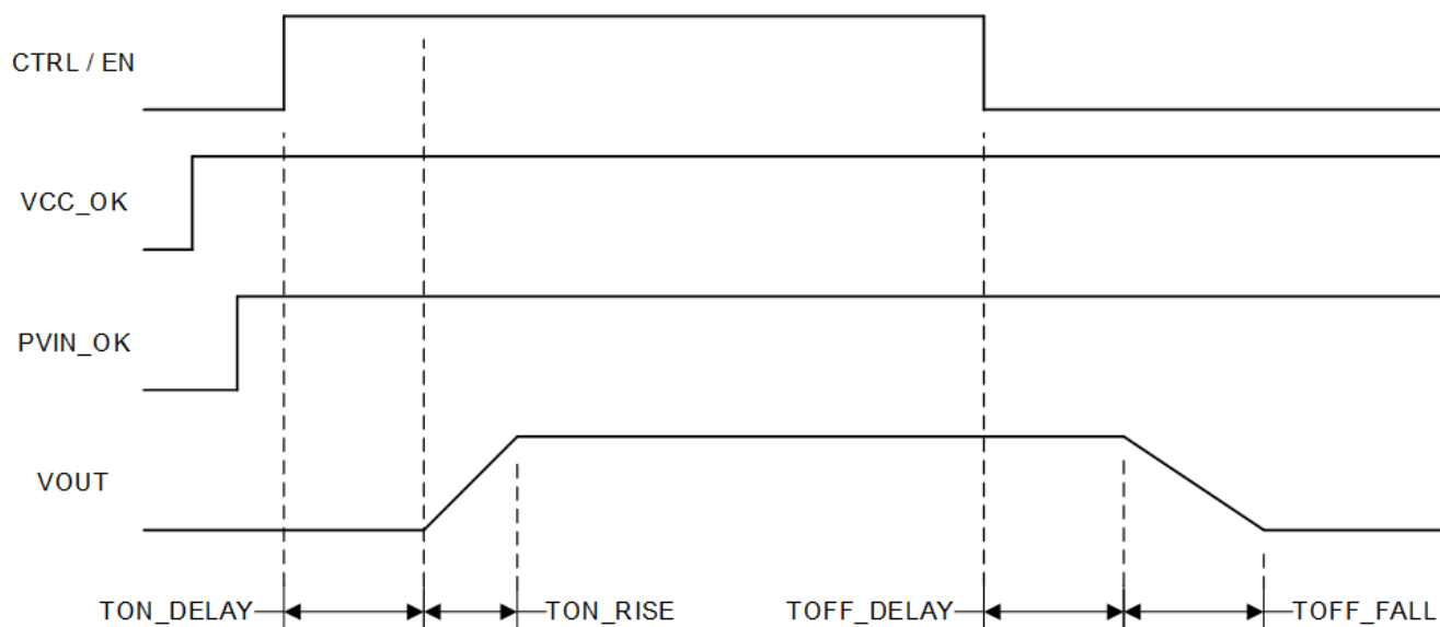
Figure 6-4. TPS546B25 Start-Up and Shutdown
