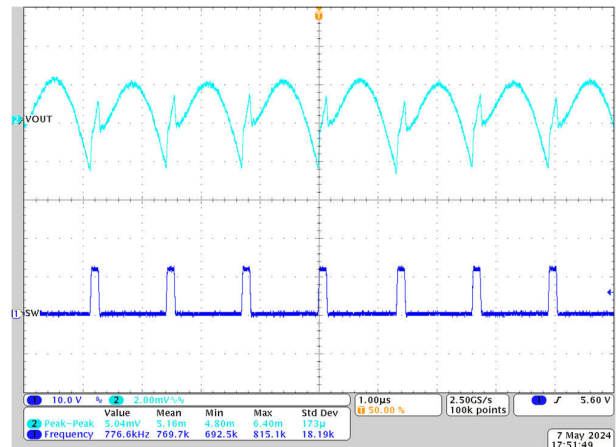
Figure 8-3. Output Voltage Ripple, 1.2V Vout, 800kHz FCCM, 25A Load
