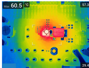
Figure 8-6. Thermal Characteristics, 800kHz FCCM, Internal LDO, 25A Load
