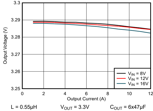
Figure 7-4. Load Regulation
