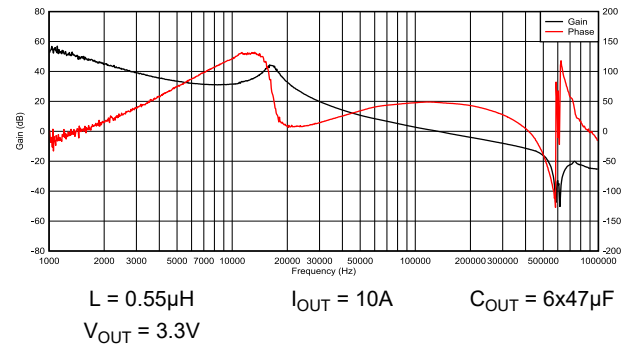
Figure 7-7. Frequency Response
