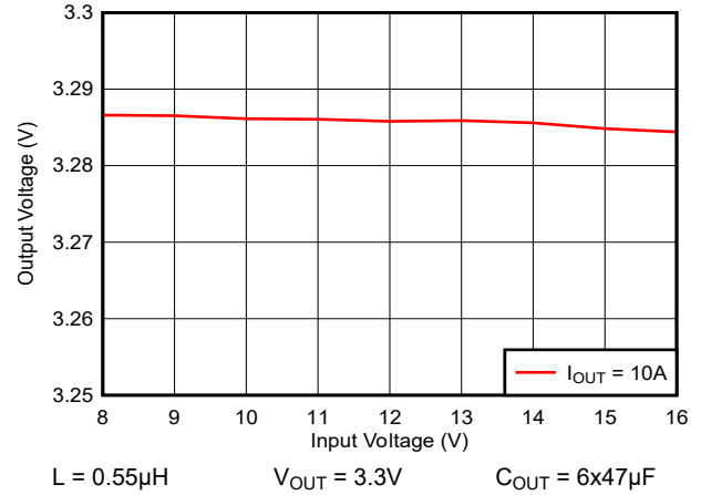
Figure 7-5. Line Regulation
