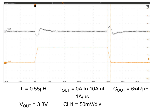
Figure 7-6. Load Transient
