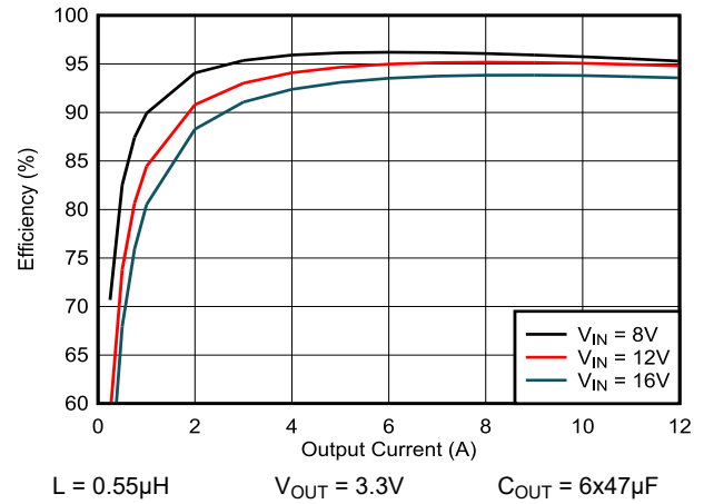
Figure 7-3. Efficiency - FCCM Mode
