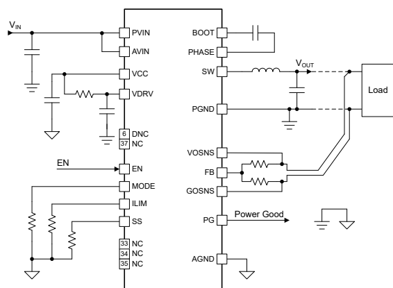
Simplified Schematic
