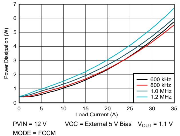
Figure 6-4. Power Dissipation vs Output Current
