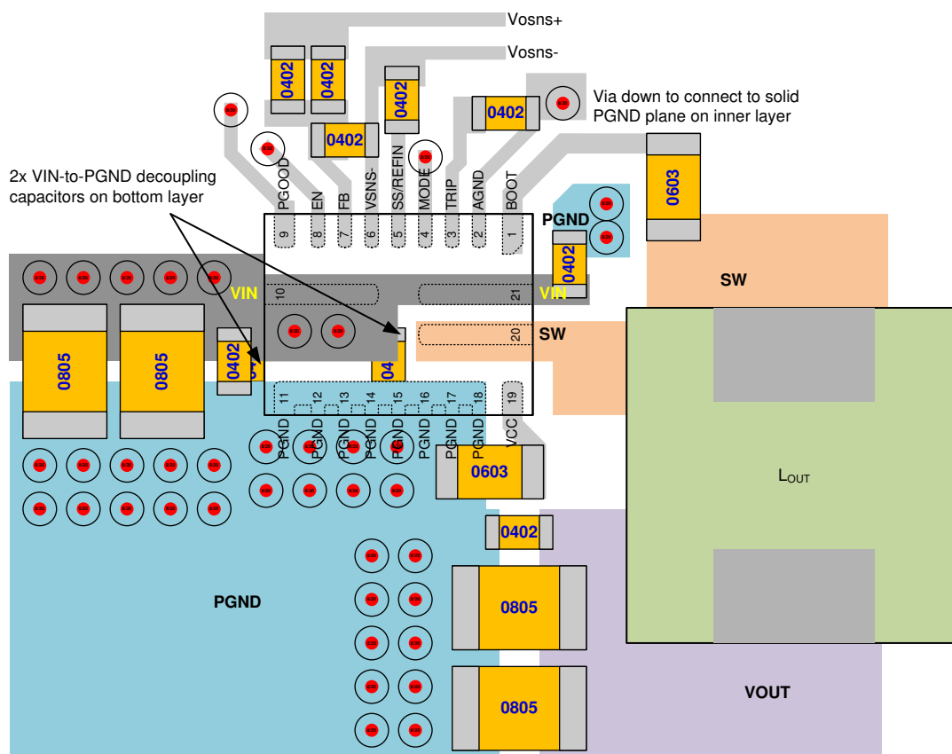
Figure 10-1. Layout Recommendation
