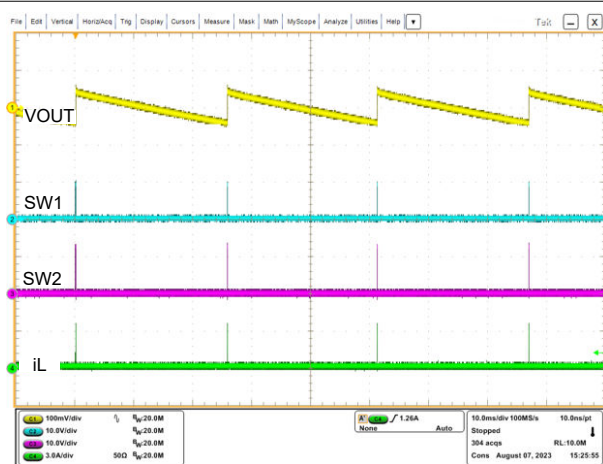
Figure 8-7. Switching Waveforms in V_{IN} = 9\text{ V} , V_{OUT} = 12\text{ V} , I_O = 0\text{ A} , PFM
