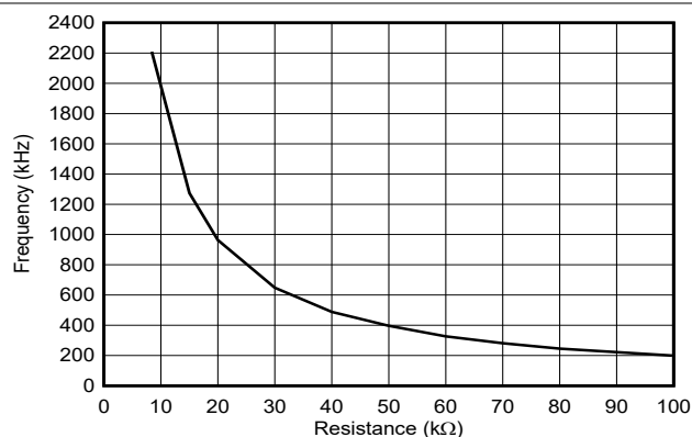
Figure 6-16. Switching Frequency vs Setting Resistance
