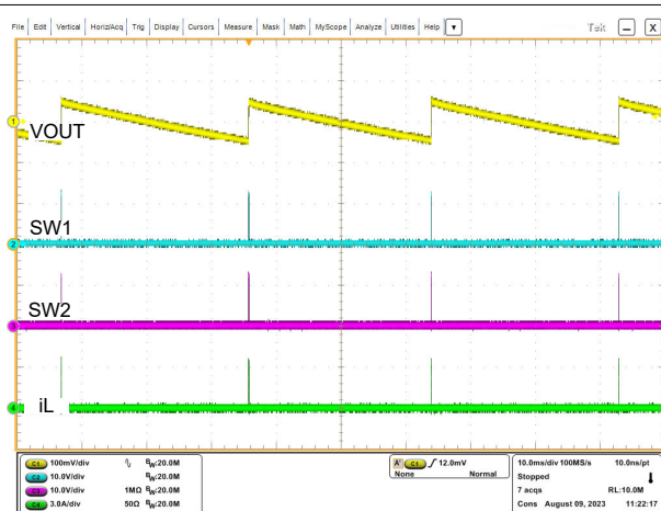
Figure 8-5. Switching Waveforms in V_{IN} = 12\text{ V} , V_{OUT} = 12\text{ V} , I_O = 0\text{ A} , PFM
