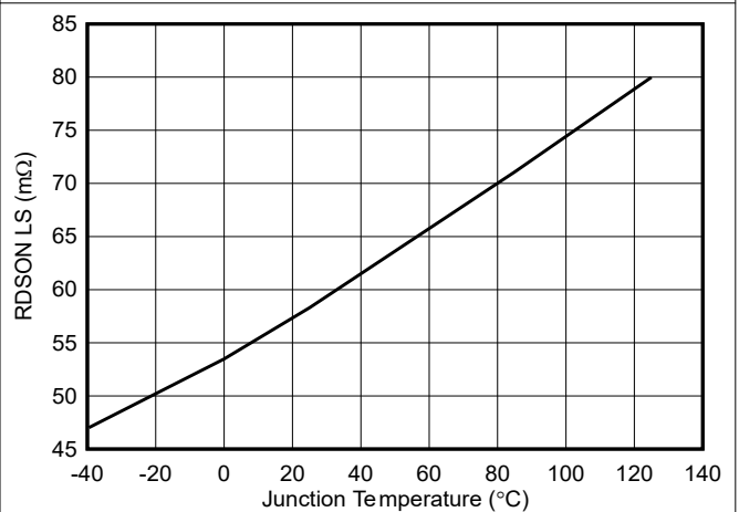
Figure 5-6. High-Side Rdson
