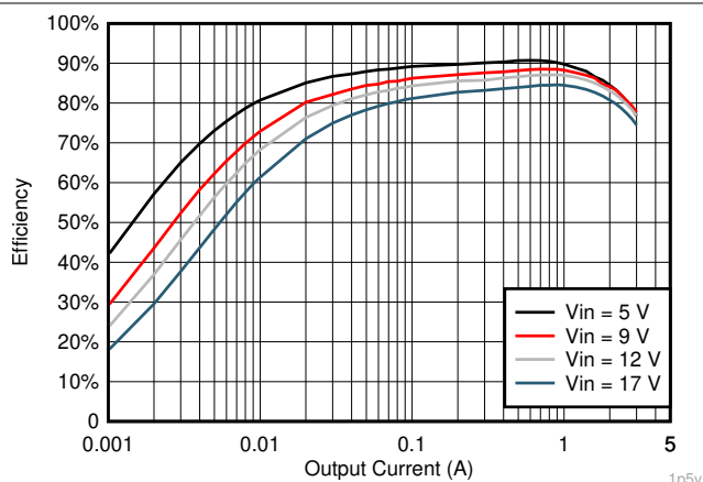
Figure 7-11. V_{OUT} = 1.5 V Efficiency, L = 1.5 \mu\text{H}
