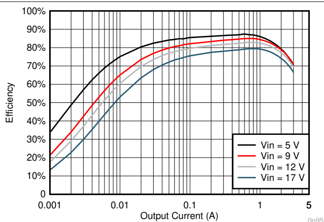
Figure 7-9. V_{OUT} = 0.95 V Efficiency, L = 1.2 \mu\text{H}
