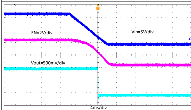
Figure 8-18. Start-Up with V_{IN} Falling, I_{OUT} = 5 A
