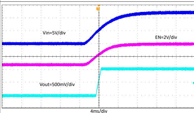
Figure 8-17. Start-Up with V_{IN} Rising, I_{OUT} = 5 A
