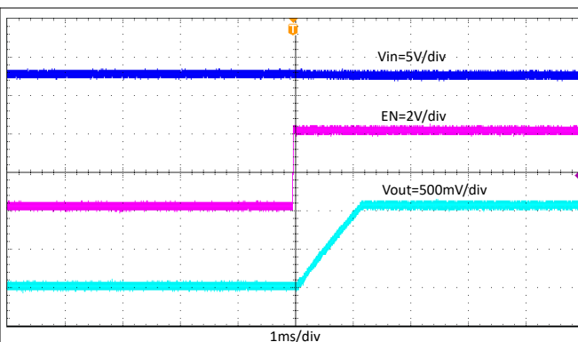
Figure 8-15. Start-Up Through EN, I_{OUT} = 5 A
