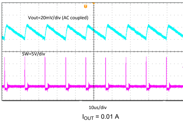
Figure 7-12. TPS566231 Output Voltage Ripple
