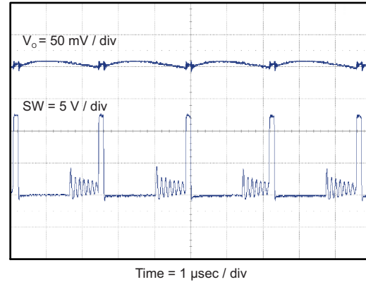
Figure 14. DCM VOLTAGE RIPPLE AT OUTPUT (IO = 30 mA)
