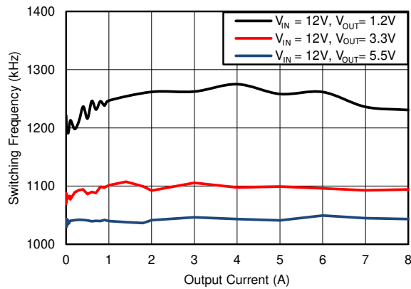
Figure 6-19. F_{SW} Load Regulation, Mode = FCCM, F_{SW} = 1200kHz
