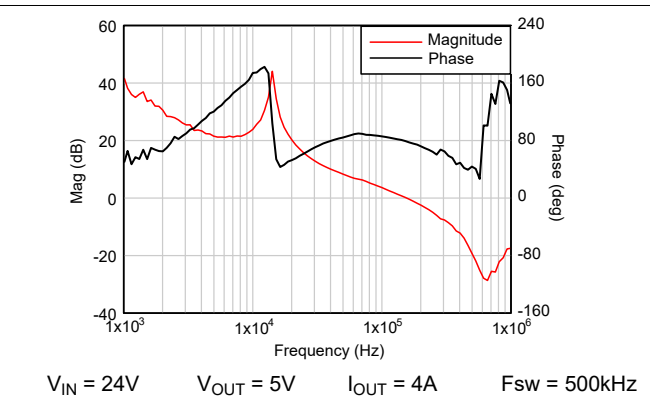
Figure 7-5. Bode Plot
