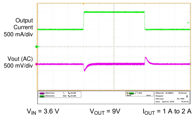
Figure 9-7. Load Transient
