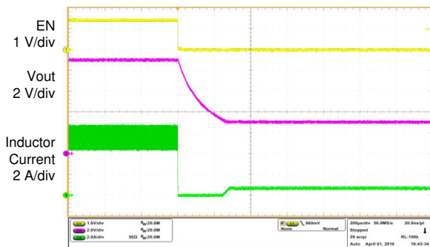
Figure 9-6. Shutdown Waveforms
