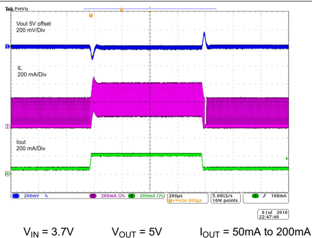
Figure 8-6. Load Transient
