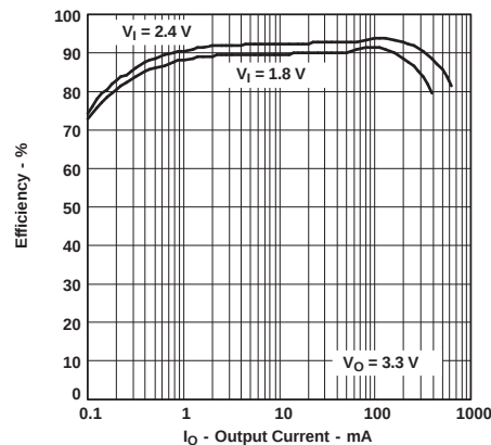
Figure 4. TPS61121 Boost Converter Efficiency vs Output Current
