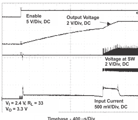
Figure 23. TPS61121 Boost Converter Start-up After Enable
