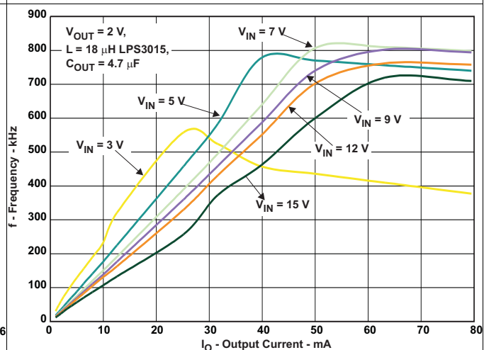
Figure 4. Switch Frequency vs Output Current I_{OUT} ( V_{OUT} = 2 V )
