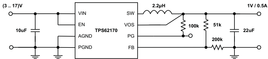
Figure 40. 1-V and 0.5-A Power Supply
