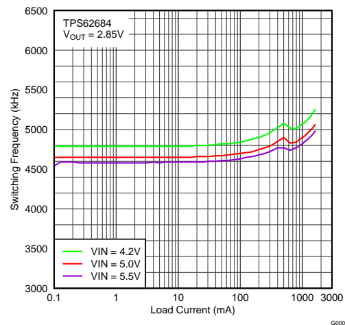
Figure 18. PWM Switching Frequency Vs Load Current
