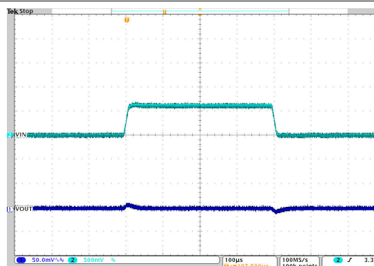
Figure 10-39. Line Transient Response
