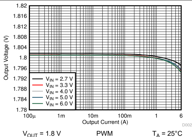
Figure 10-15. Output Voltage Versus Output Current
