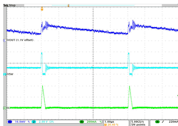
Figure 9-8. Switching Frequency
