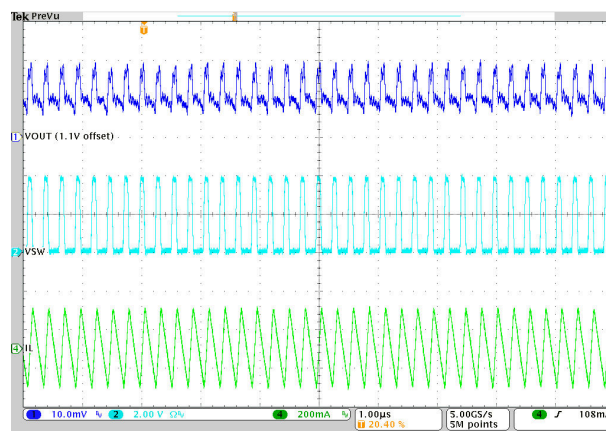
Figure 9-9. Switching Frequency
