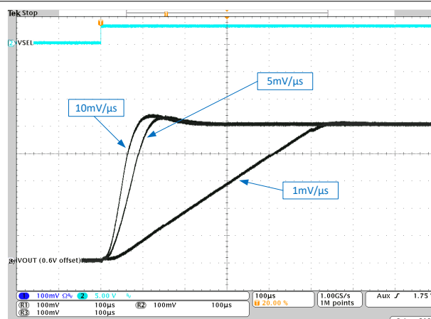
Figure 9-11. PWM-Mode Operation
