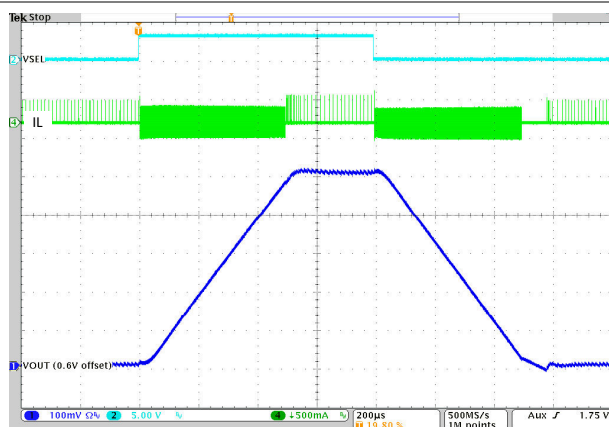
Power Save Mode is active Figure 9-15. FPWM-Mode During V_{OUT} Change Enabled
