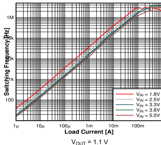
Figure 9-9. Switching Frequency
