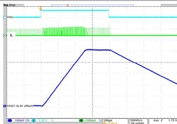
Power Save Mode is active Figure 9-14. Standard Operation: V_{OUT} Change
