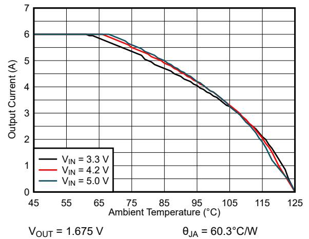
Figure 9-11. Thermal Derating
