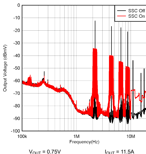
Figure 9-19. Spread Spectrum Operation
