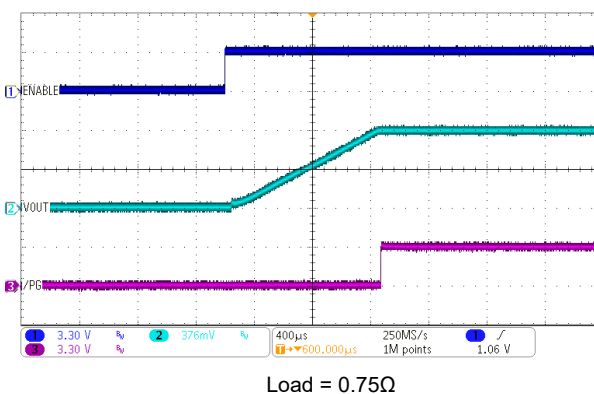
Figure 9-21. Start-Up Using the EN Pin
