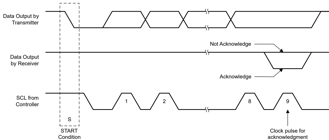
Figure 7-18. Acknowledge on the I²C Bus
