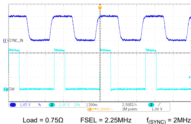
Figure 9-20. Synchronization to an External Clock
