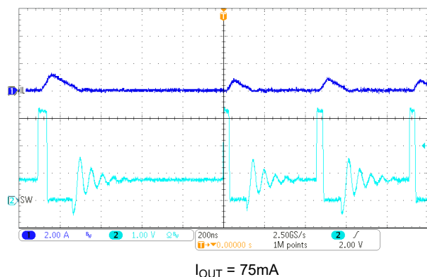
Figure 9-18. PFM Operation
