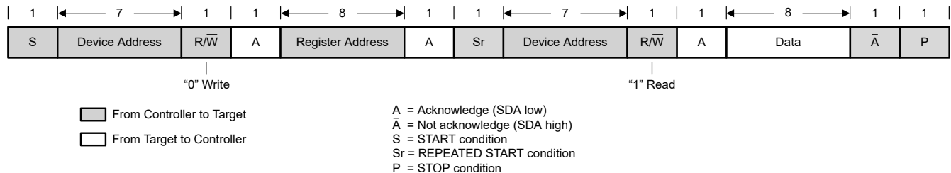
Figure 7-21. "Read" Data Transfer Format in Standard, Fast, Fast Plus Modes
