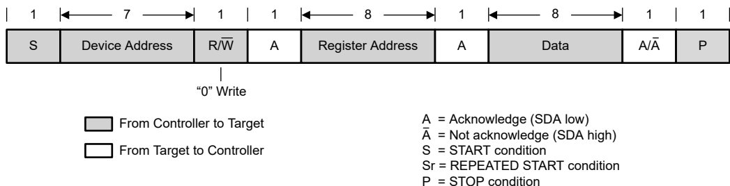
Figure 7-20. "Write" Data Transfer Format in Standard, Fast, Fast Plus Modes
