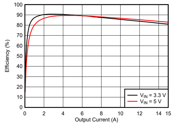
Efficiency vs Output Current V OUT = 0.75V, FPWM, f sw = 2.25MHz
