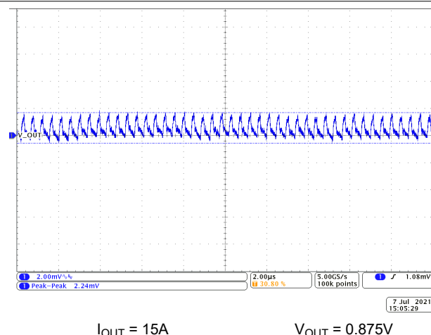
Figure 9-13. Output Voltage Ripple
