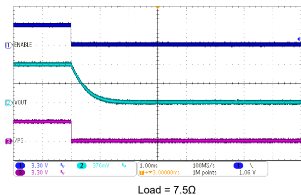
Figure 9-22. Shutdown Using the EN Pin (Discharge Enabled)
