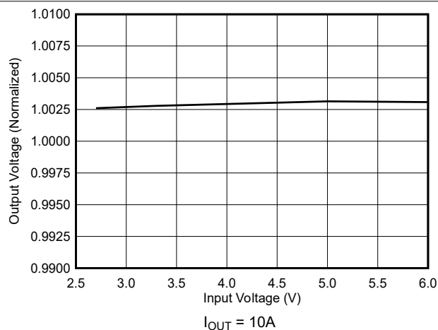
Figure 9-12. Line Regulation
