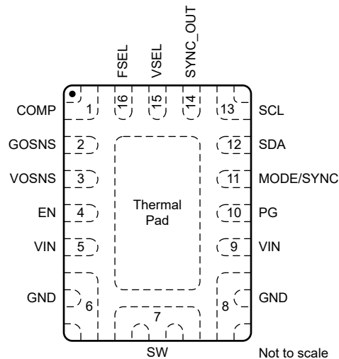
Figure 5-1. 16-Pin RXS VQFN Package (Top View)
