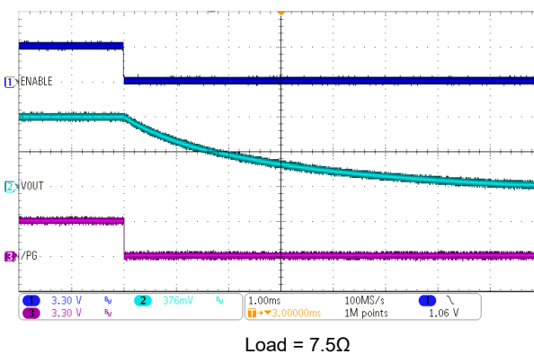
Figure 9-23. Shutdown (Discharge disabled)
