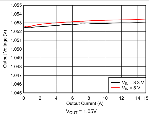
Figure 9-11. Load Regulation
