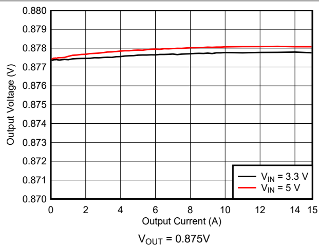
Figure 9-9. Load Regulation
