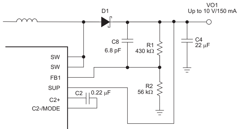
Figure 16. Feedforward Capacitor
