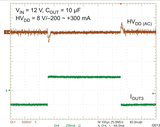
Figure 6-12. SYNCHRONOUS BUCK ( HV_{DD} ) LOAD TRANSIENT RESPONSE
