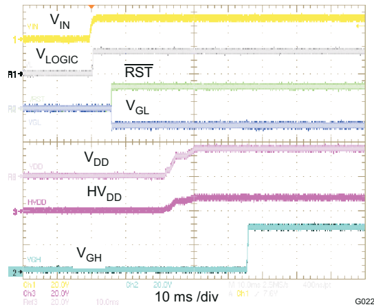
Figure 6-22. STARTUP SEQUENCING
