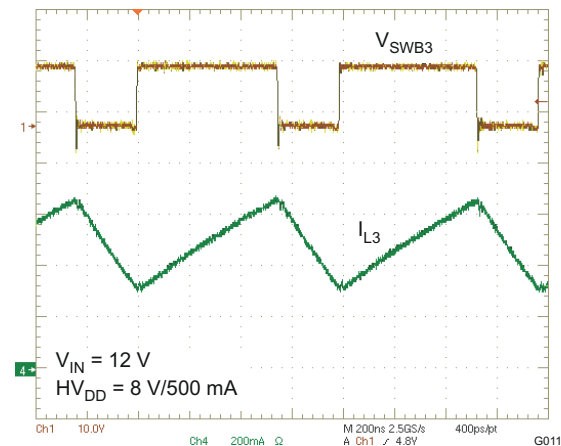
Figure 6-10. SYNCHRONOUS BUCK ( HV_{DD} ) PWM SWITCHING – HEAVY LOAD (SOURCE)
