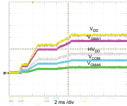
Figure 6-23. STARTUP SEQUENCING
