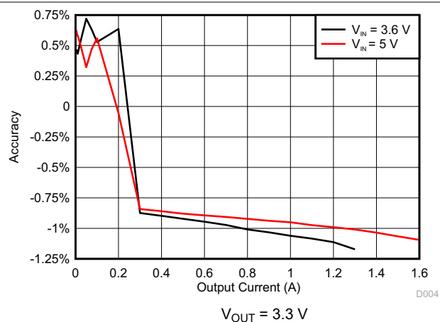
Figure 6-4. DCDC4 Accuracy
