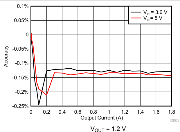
Figure 6-3. DCDC3 Accuracy
