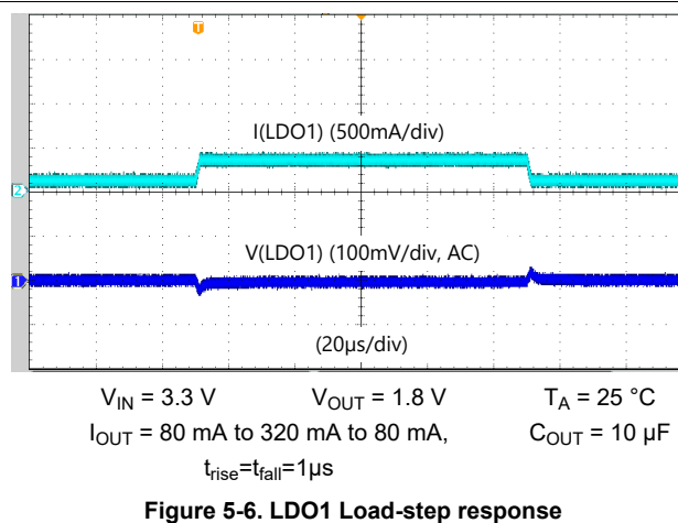
Figure 5-6. LDO1 Load-step response
