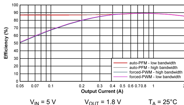
Figure 5-2. Efficiency BUCK23
