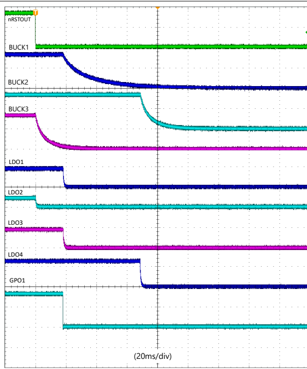
Figure 7-9. LDOs Discharge
