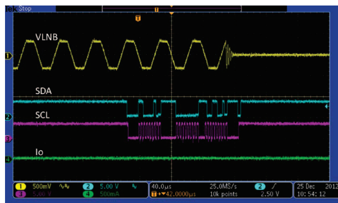
Figure 41. V_{IN} = 12\text{ V} , V_{LNB} = 13.4\text{ V} , No Loading, 22-kHz Tone Delay from I^2\text{C} SDA to Output Tone, Off
