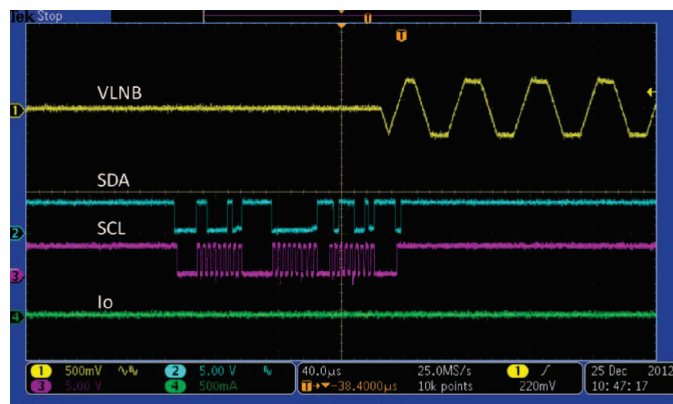
Figure 37. V_{IN} = 12\text{ V} , V_{LNB} = 13.4\text{ V} , No Loading, 22-kHz Tone Delay from I^2\text{C} SDA to Output Tone, On
