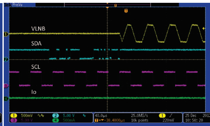
Figure 38. V_{IN} = 12\text{ V} , V_{LNB} = 13.4\text{ V} , No Loading, 22-kHz Tone Delay from I^2\text{C} Gated, EXT M Provides 22 kHz to Output Tone, On
