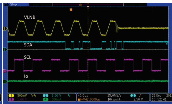
Figure 42. V_{IN} = 12\text{ V} , V_{LNB} = 13.4\text{ V} , No Loading, 22-kHz Tone Delay from I^2\text{C} Gated, EXT M Provides 22 kHz to Output Tone, Off
