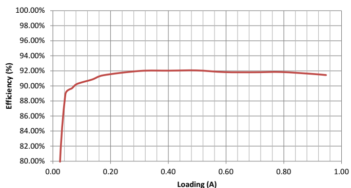
Figure 1. Efficiency ( V_{IN} = 12\text{ V} , V_{LNB} = 13.4\text{ V} )
