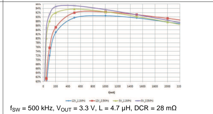
Figure 2. BUCK1 Efficiency
