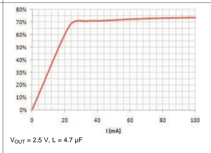
Figure 6. BUCK2 Efficiency Low-Power Enabled
