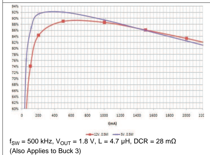
Figure 5. BUCK2 Efficiency
