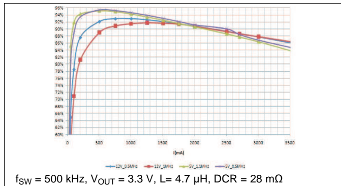
Figure 1. BUCK1 Efficiency
