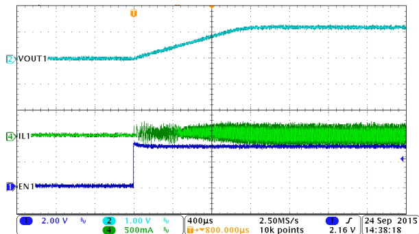
Figure 8-27. PWM Mode, Buck1, Soft-Start with No Load
