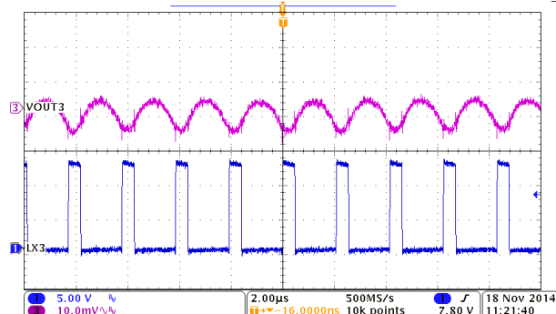
Figure 8-8. BUCK3, Output Voltage Ripple
