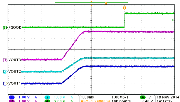
Figure 8-18. PGOOD
