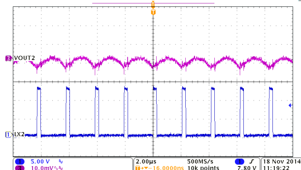
Figure 8-7. BUCK2, Output Voltage Ripple
