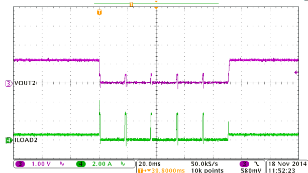
Figure 8-16. BUCK2, Hiccup and Recovery
