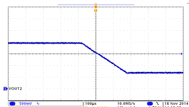
Figure 8-20. VID2 from 7F to 00, SR = 10 mV/Cycle
