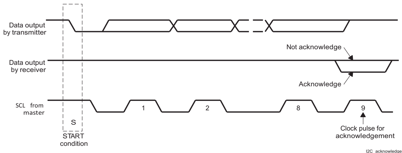
Figure 6-13. Acknowledge on the I 2 C Bus
