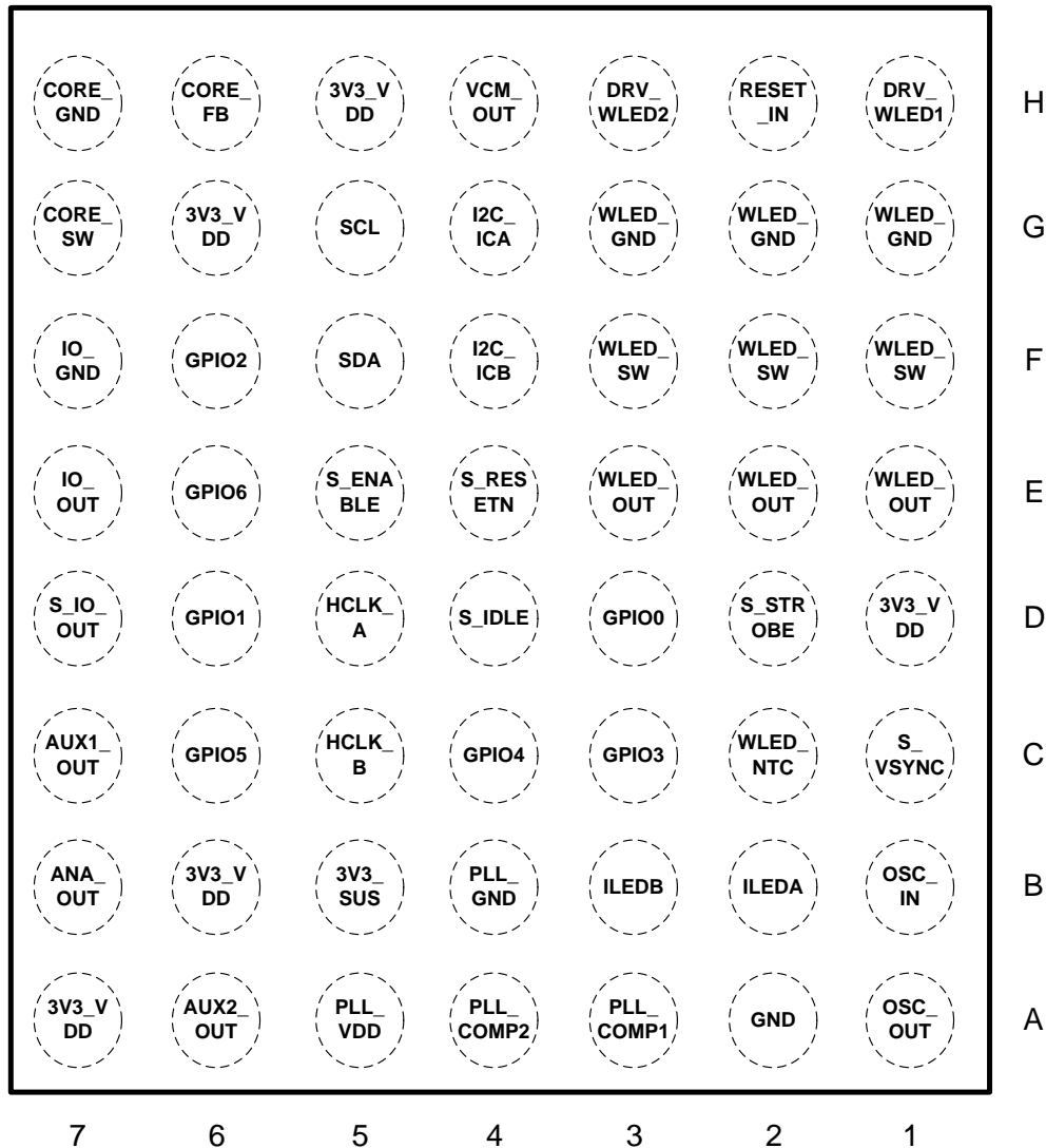
Pin Functions
