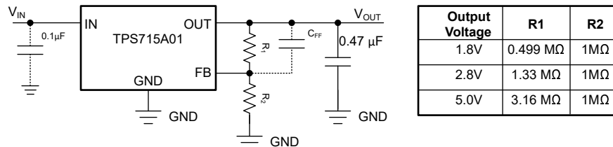
Figure 7-2. TPS715A01 Adjustable LDO Regulator Programming
