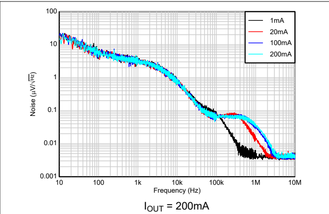
Figure 5-62. TPS72325 Total Noise vs V_{IN} (10Hz to 10MHz) (New chip)
