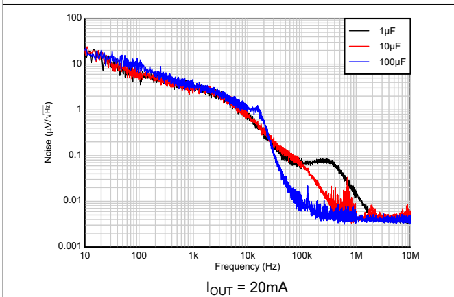
Figure 5-65. TPS72325 Total Noise vs C_{OUT} (10Hz to 10MHz) (New chip)
