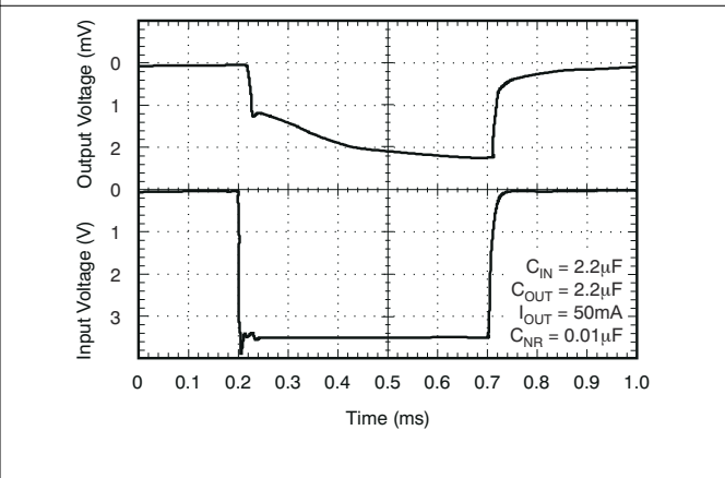
Figure 5-48. TPS72325 Start-Up Response (legacy chip)
