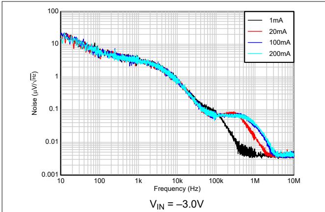
Figure 5-61. TPS72325 Total Noise vs I_{OUT} (10Hz to 10MHz) (New chip)
