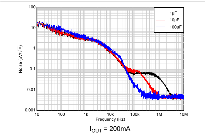
Figure 5-64. TPS72325 Total Noise vs C_{OUT} (10Hz to 10MHz) (New chip)
