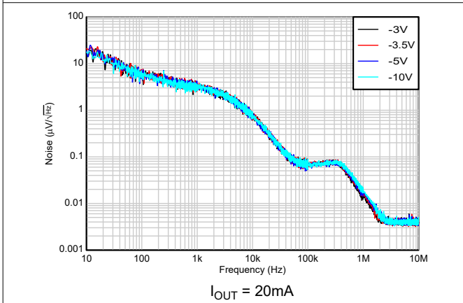
Figure 5-63. TPS72325 Total Noise vs V_{IN} (10Hz to 10MHz) (New chip)
