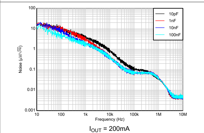
Figure 5-66. TPS72301 Total Noise vs C_{FF} (10Hz to 10MHz) (New chip)
