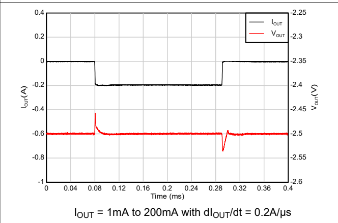
Figure 5-46. TPS72325 Load Transient Response (new chip)
