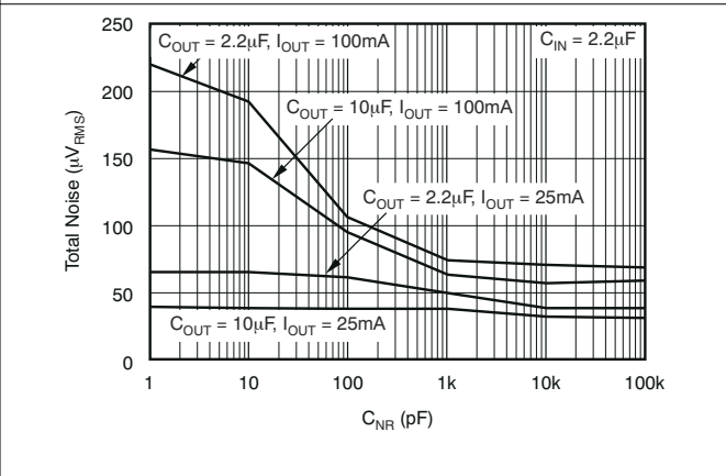
Figure 5-58. TPS72325 Total Noise vs C_{NR} (10Hz to 100kHz) (legacy chip)
