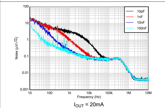
Figure 5-60. TPS72325 Total Noise vs C_{NR} (10Hz to 10MHz) (New chip)
