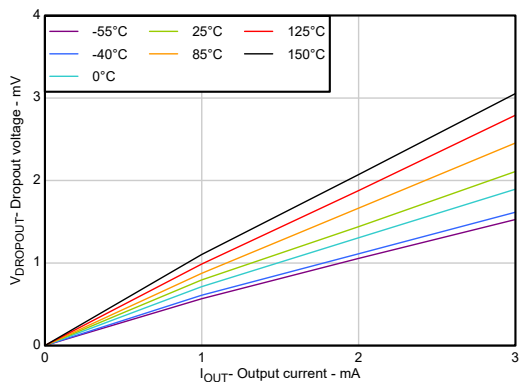
Figure 5-7. Dropout Voltage vs Output Current (legacy chip)
