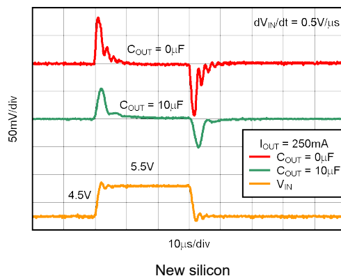
Figure 5-38. TPS73233-Q1 Line Transient Response
