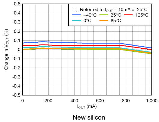
Figure 5-2. Load Regulation
