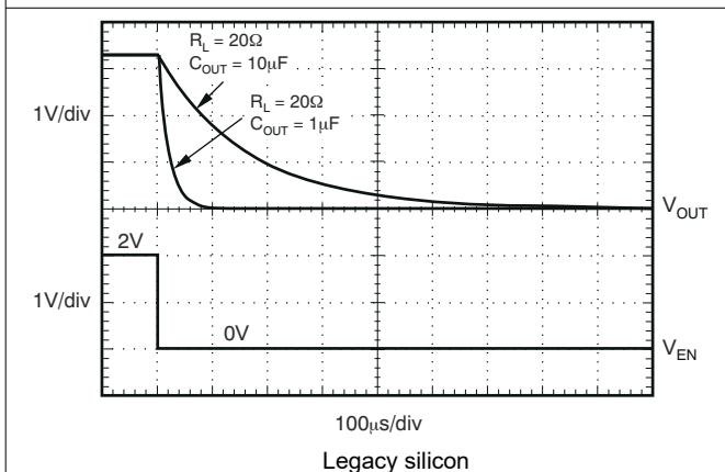
Figure 5-41. TPS73701-Q1 Turn-Off Response
