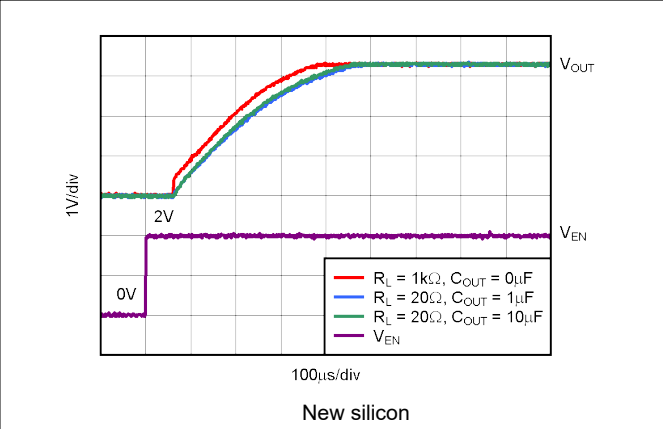
Figure 5-40. TPS73701-Q1 Turn-On Response
