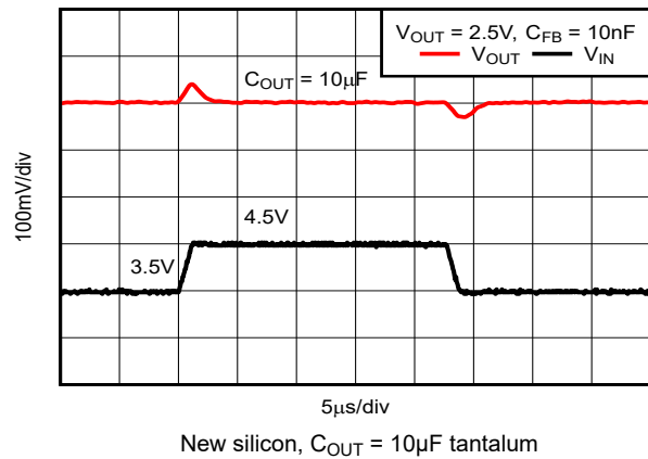
Figure 5-52. TPS73701-Q1 Line Transient, Adjustable Version
