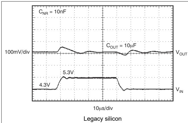
Figure 5-37. TPS73733-Q1 Line Transient Response
