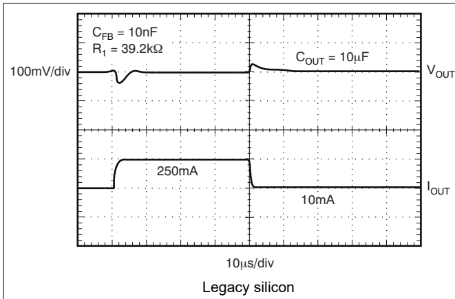
Figure 5-49. TPS73701-Q1 Load Transient, Adjustable Version
