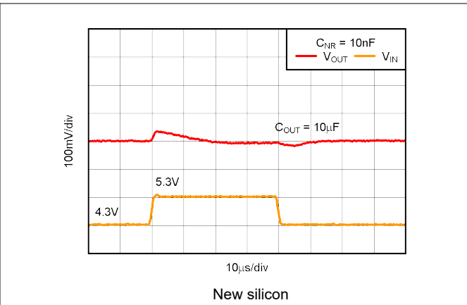
Figure 5-38. TPS73733-Q1 Line Transient Response
