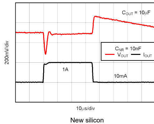
Figure 5-36. TPS73733-Q1 Load Transient Response
