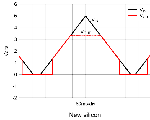
Figure 5-44. TPS73701-Q1, V_{OUT} = 3.3\text{V} Power-Up and Power-Down
