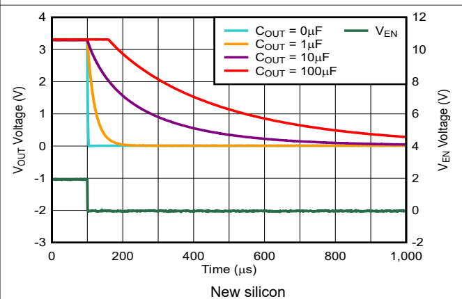
Figure 5-42. TPS73701-Q1 Turn-Off Response
