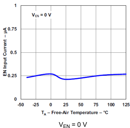
Figure 5-9. EN Input Current vs Temperature
