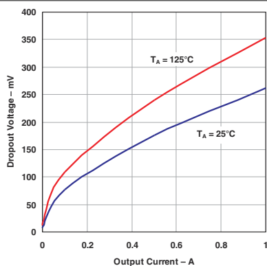
Figure 5-1. Dropout Voltage vs Output Current
