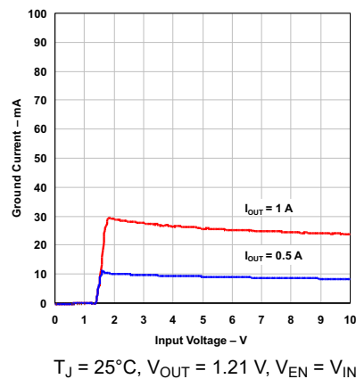
Figure 5-6. Ground Current vs Input Voltage
